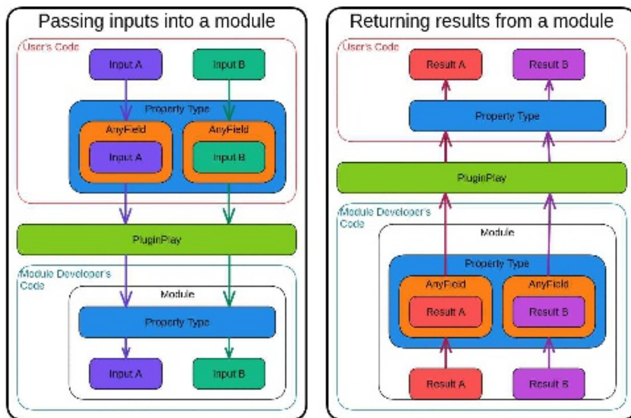
FIG. 4. Illustration of how data traverses module boundaries in PluginPlay. See Section III C for more details.
