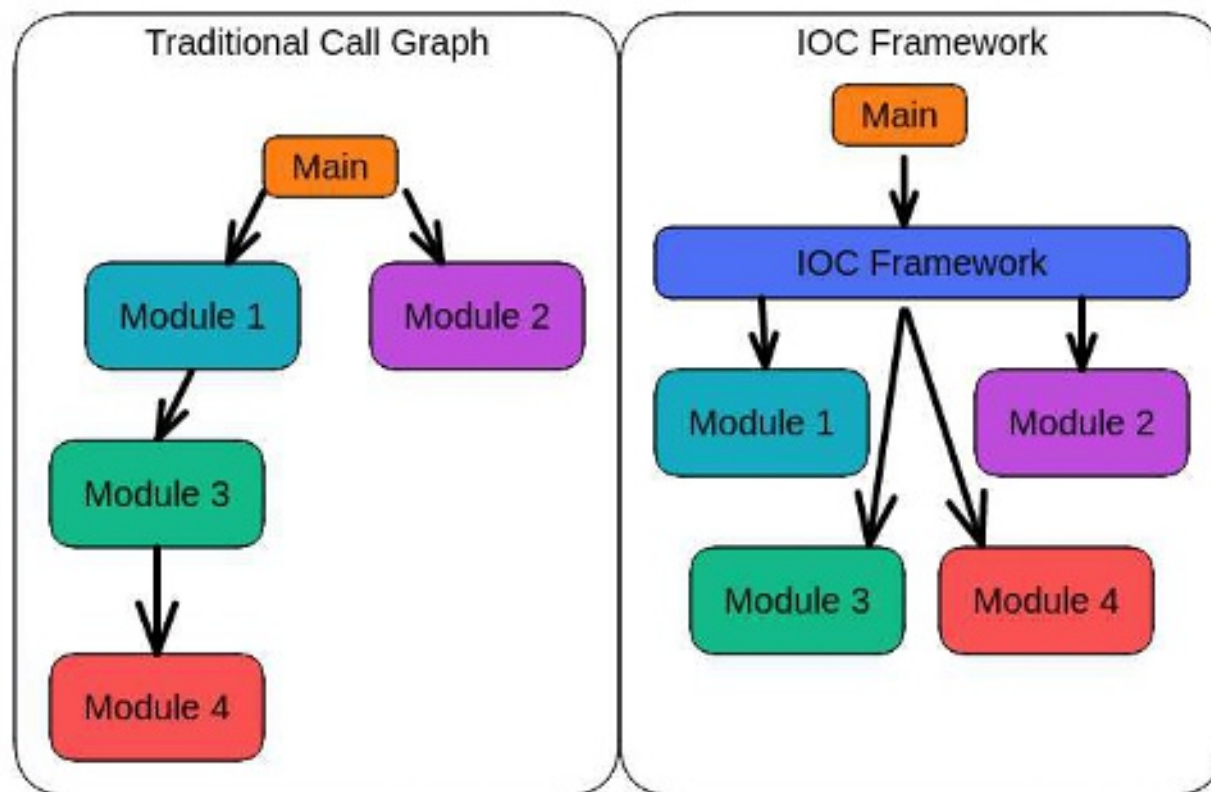
FIG. 1. Difference between a normal package and a package powered by an IOC framework. In both panels modules are called in a top-to-bottom, left-to-right ordering.
