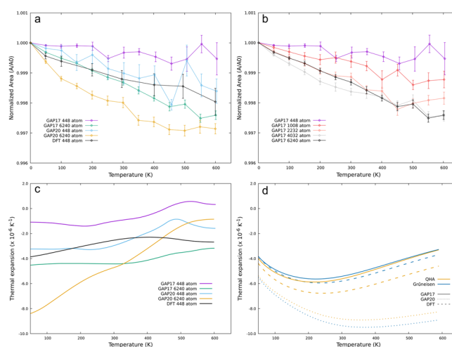
Figure 3. (a) Normalized area versus simulation temperature for molecular dynamics calculations with DFT, GAP17, and GAP20 models. (b) Normalized area versus simulation temperature for molecular dynamics calculations GAP17 model w.r.t system size. (c) Calculated thermal expansion coefficients of graphene by MD simulations with DFT, GAP17, and GAP20 models. (d) Calculated thermal expansion coefficients of graphene QHA and Grüneisen framework with GAP models and DFT.
