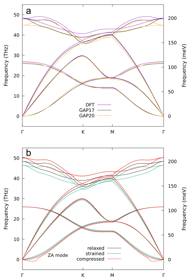
Figure 1. (a) Phonon dispersion relations of relaxed graphene monolayers by DFT, GAP17, and GAP20 models. (b) Phonon dispersion relations of relaxed, 1% strained, and 1% compressed graphene monolayers by GAP17 model compared to DFT. Dashed lines show the corrected phonon curves of the compressed case.
