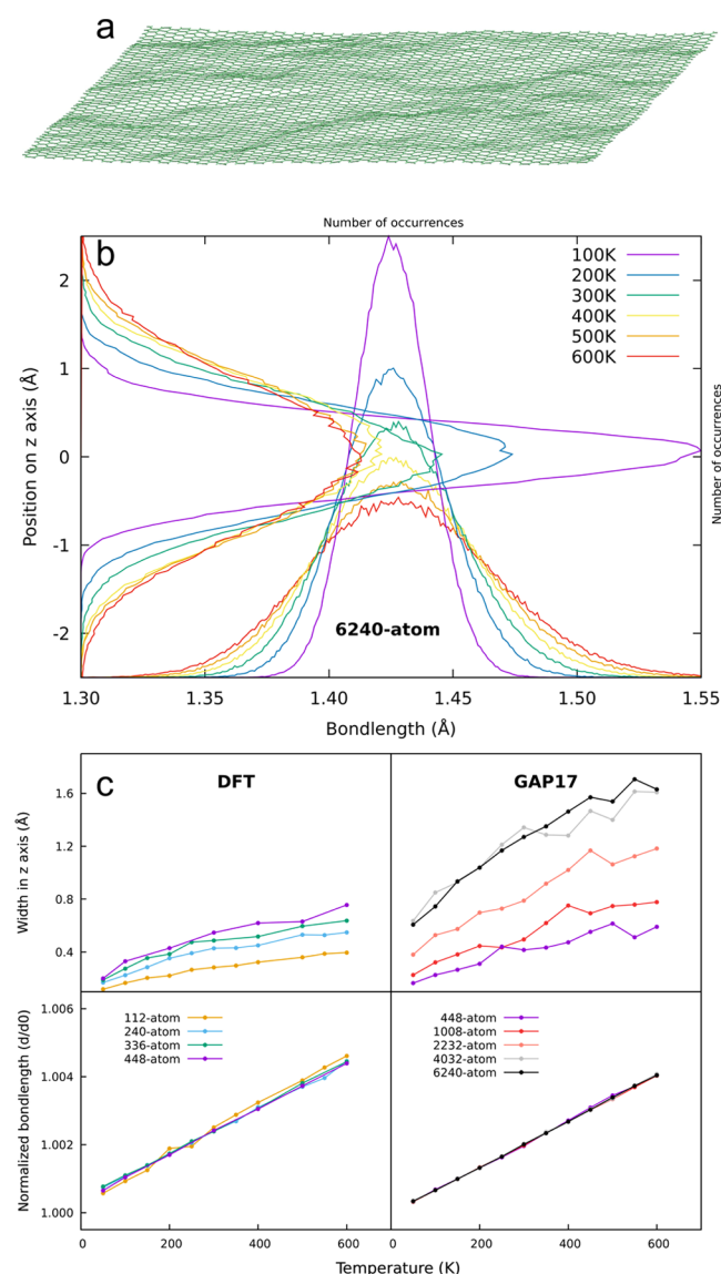
Figure 4. (a) Side view of graphene monolayer within an MD frame demonstrating the rippling behavior. (b) Structural analysis of 6240-atom graphene system obtained from MD simulations with the GAP17 model. The bond length distribution is given in the horizontal axis, while the position distribution on the z-axis is given in the vertical axis against the number of occurrences. (c) Normalized bond length versus temperature and rippling width versus temperature graphs of graphene obtained from MD simulations. Rippling width is calculated as 2\sigma from the standard deviation of the position distribution on the z-axis, and the bond lengths are normalized using the bond length of the relaxed system ( d_0 ).
