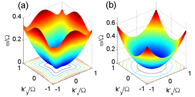
FIG. 10. (Color online) Dispersion relation of the acoustic Tkachenko modes of the rectangular lattice, Eq. (88) for \alpha=0.95 (a) and for \alpha=1.0 (b). At \alpha=1.0 , the dispersion relation becomes isotropic. The similarity between (a) and Fig. 7(b) is due to the second-order phase transition between square and rectangular lattices.
