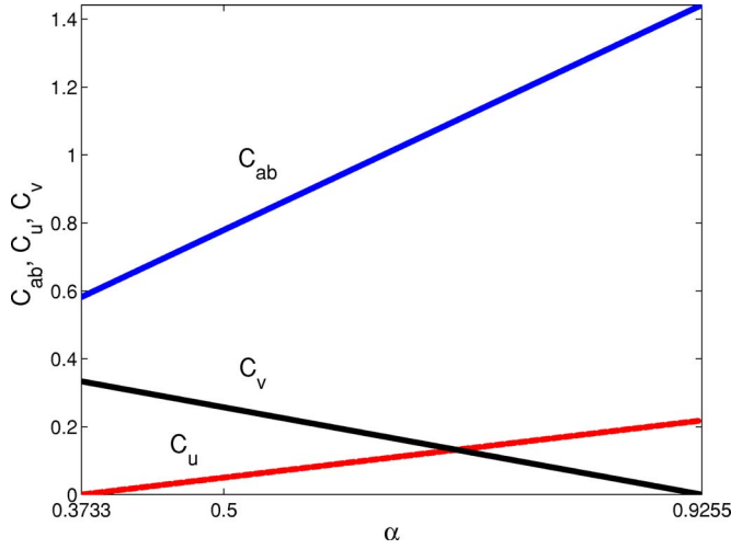
FIG. 6. (Color online) Elastic constants ( C_{ab}, C_u, C_v ) of square lattice, Eqs. (67) and (75). As the components attract each other more, C_{ab} increases linearly. Both limits of \alpha lead to second-order phase transitions. C_u and C_v vanish at \alpha=0.3733 and \alpha=0.9255 , respectively.
