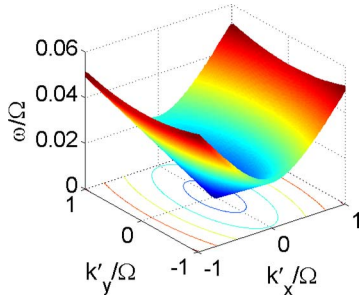
FIG. 9. (Color online) Dispersion relation of the optical Tkachenko mode of the rectangular lattice, Eq. (94), for \alpha=0.95 , gn/\Omega=0.1 . The underlying contour plot reflects the symmetry of the rectangular lattice.
