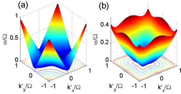
FIG. 7. (Color online) Dispersion relation of the acoustic Tkachenko modes for the square lattice, Eq. (72), for \alpha=0.4 (a), and \alpha=0.85 (b). Underlying contour plots are given to illustrate the anisotropy of the modes.
