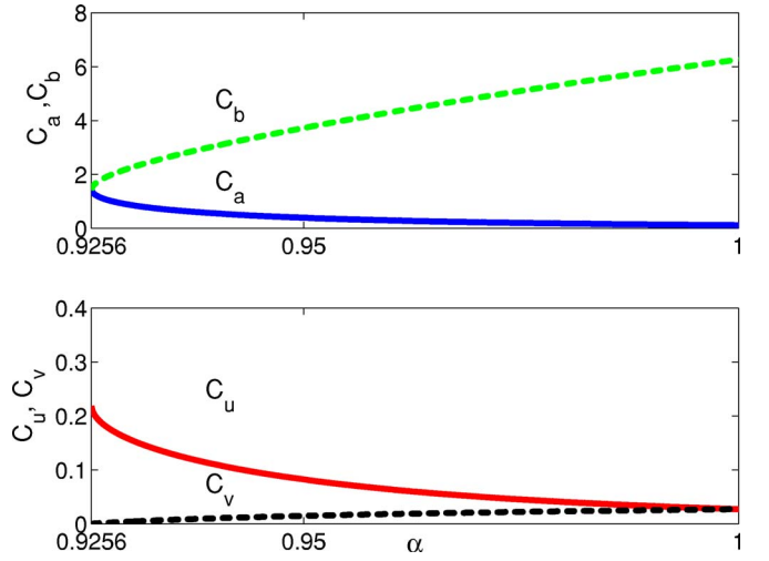
FIG. 8. (Color online) Elastic constants ( C_a, C_b, C_u, C_v ) of rectangular lattice. The upper figure shows optical elastic constants ( C_a, C_b ). As \alpha \rightarrow 1 , C_a vanishes. The lower figure shows acoustic elastic constants ( C_u, C_v ). As \alpha \rightarrow 1 , C_u \rightarrow C_v and there remains only one acoustic elastic constant similar to the one-component triangular lattice.
