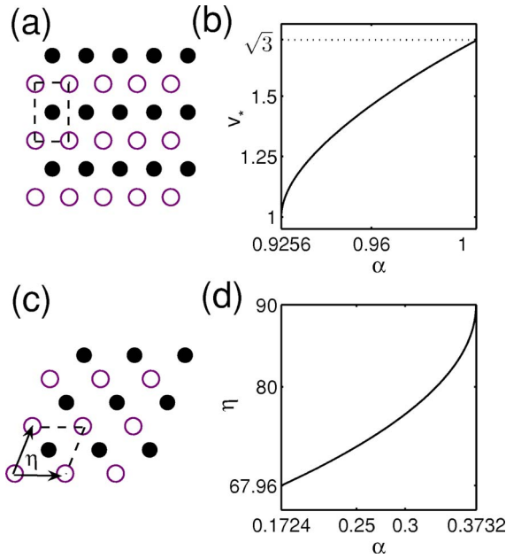
FIG. 2. (Color online) (a) Lattice geometry for a rectangular lattice; a unit cell is shown with dashed lines. (b) Change of the aspect ratio of the rectangle v_* with respect to interaction strength \alpha . The unit cell grows in the y direction as \alpha \rightarrow 1 . At \alpha = 1 , v_* = \sqrt{3} . (c) Lattice geometry of a rhombic lattice, dashed lines showing a unit cell. \eta is twice the opening angle of the rhombic unit cell. (d) Plot of \eta vs \alpha for the rhombic lattice. As \alpha \rightarrow 0.3732 , \eta \rightarrow 90^\circ , and the rhombus continuously changes to a square. At \alpha = 0.1724 , \eta makes a jump from 60^\circ to 67.958^\circ .
