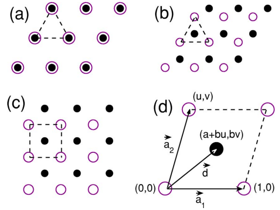
FIG. 1. (Color online) Lattice geometry for an overlapped triangular lattice (a), an interlaced triangular lattice (b), and a square lattice (c). Unit cells are shown with dashed lines. (d) Unit-cell geometry for an arbitrary lattice. White and black dots represent vortices of different components. Definitions of a, b, u, v are given in Sec. II.
