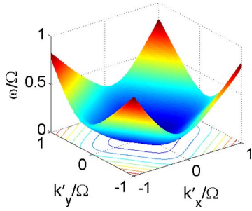
FIG. 12. (Color online) Dispersion relation of the acoustic Tkachenko mode of the rhombic lattice, Eq. (104), for \alpha=0.2 . The anisotropy reflects the twofold symmetry of the rhombic lattice (see Fig. 13).
