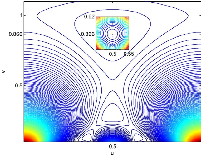
FIG. 3. (Color online) Contour plot of the energy for a one-component triangular lattice, Eq. (15). The inset is a closer view around the equilibrium point. Circular contours indicate that quadratic fit of Eq. (16) is possible.
