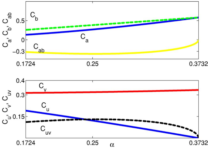
FIG. 11. (Color online) Optical elastic constants [upper, Eq. (108)] and acoustic elastic constants [lower, Eq. (101)] of rhombic lattice with respect to \alpha . As \alpha \rightarrow 0.3732 , C_a \rightarrow C_b , and C_u, C_v vanish, leaving two optical elastic constants, and one acoustic elastic constant for the square lattice. In the opposite limit \alpha \rightarrow 0.1724 , six elastic constants remain due to the discontinuity in the transition to interlaced triangular lattice.
