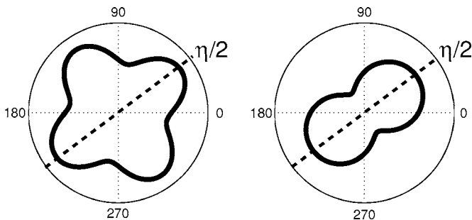
FIG. 13. Polar plot of the frequency of the acoustic [left, Eq. (104)] and the optical [right, Eq. (111)] Tkachenko modes for the rhombic lattice ( k=0.1 , gn/\Omega=0.1 , \alpha=0.2 ). \eta/2 is the opening angle of the rhombic unit cell at \alpha=0.2 .
