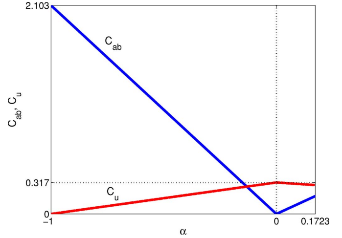
FIG. 4. (Color online) Elastic constants ( C_{ab}, C_u ) of overlapped ( -1 < \alpha < 0 ) and interlaced ( 0 < \alpha < 0.1723 ) triangular lattices with respect to \alpha . As the attraction between the components increases ( \alpha \rightarrow -1 ), C_{ab} increases, and C_u decreases linearly. When there is no interaction between components ( \alpha=0 ), C_{ab}=0 which causes the discontinuity in the transition to interlaced triangular lattice. At \alpha=0 , the value of C_u is equal to the shear modulus of a one-component vortex lattice.
