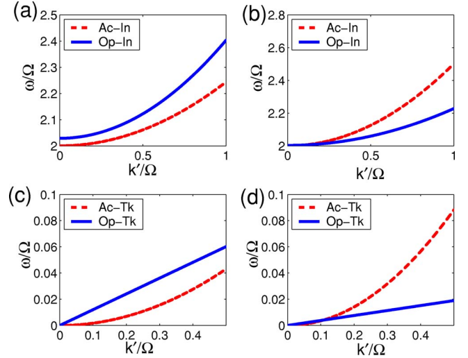
FIG. 5. (Color online) Spectrum for overlapped triangular lattice, (a), (c), at \alpha = -0.5 , and interlaced triangular lattice, (b), (d), at \alpha = 0.1 . k' and \omega are scaled to rotation frequency \Omega , and gn/\Omega = 0.1 . Dispersion relations are the same for both lattice types, Eqs. (53) and (59). However, the elastic constants are different (see Fig. 4). Both acoustic and optical inertial modes, (a), (b), are gapped. For both lattices optical Tkachenko modes are linear while acoustic Tkachenko modes are quadratic in k .
